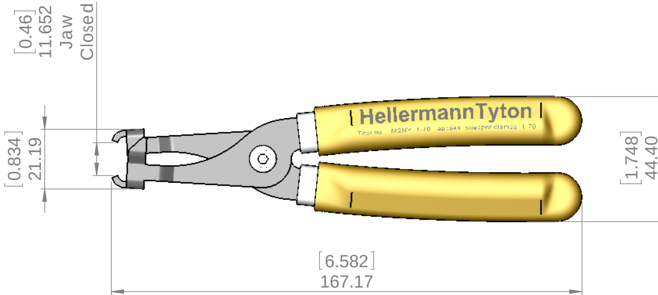
Jaws Closed
