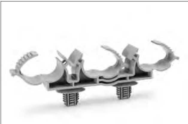
Fixing element for parallel routing of three harnesses or tubes (12.2 - 18.0mm).
