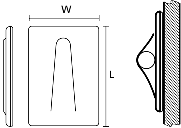
SAC-Series Self Adhesive Clip
