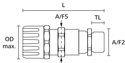
HeliaGuard fittings, forskruning, lige
