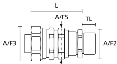
HelaGuard fitting, lige
