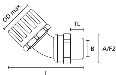
HeliaGuard fitting, 45° with swivel internal thread
