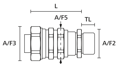
HelaGuard compression fitting, straight cable gland
