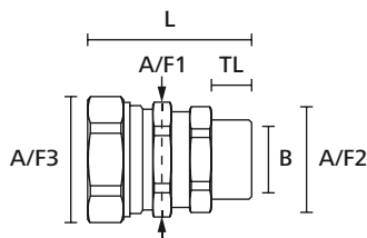
HelaGuard compression fitting, straight with swivel external thread
