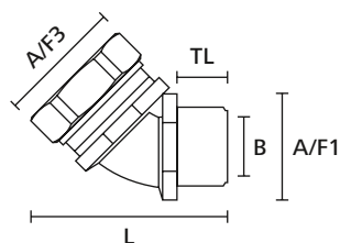
HelaGuard compression fitting, 45° with fixed external thread
