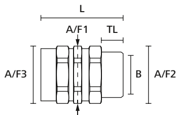
HelasGuard fitting, straight with swivel external thread
