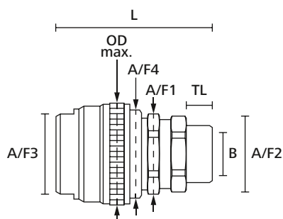
HelasGuard compression fitting, straight with swivel external thread
