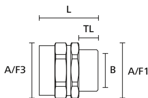
HelaGuard fitting, straight with fixed external thread
