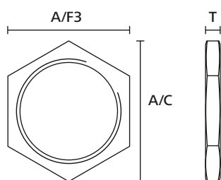
HelaGuard locknut
