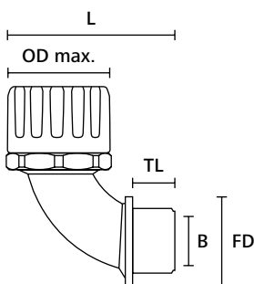
Helagaard fitting, 90° with fixed external thread
