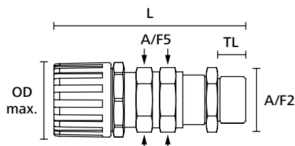
HelaGuard fitting, straight cable gland
