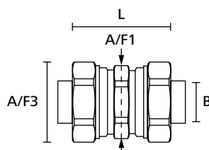
HelaGuard compression coupler
