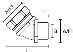
HelaGuard compression fitting, 45° with fixed external thread
