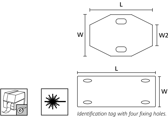
Identification tag with four fixing holes.
