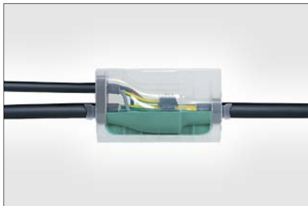
Parallel branch joint PAH-4 140/420, house connector set.
