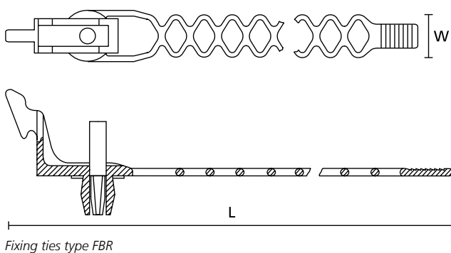
Fixing ties type FBR
