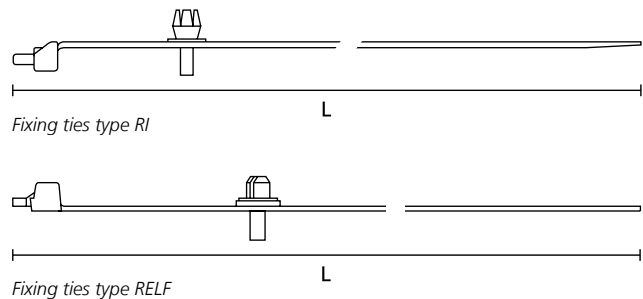
Fixing ties type RELF
